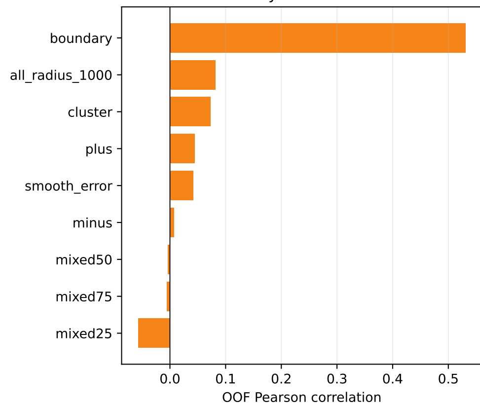
Validation stability across scenario families
