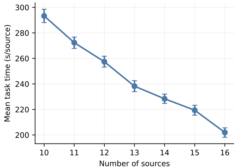
(a) Q3 sensitivity to source count
