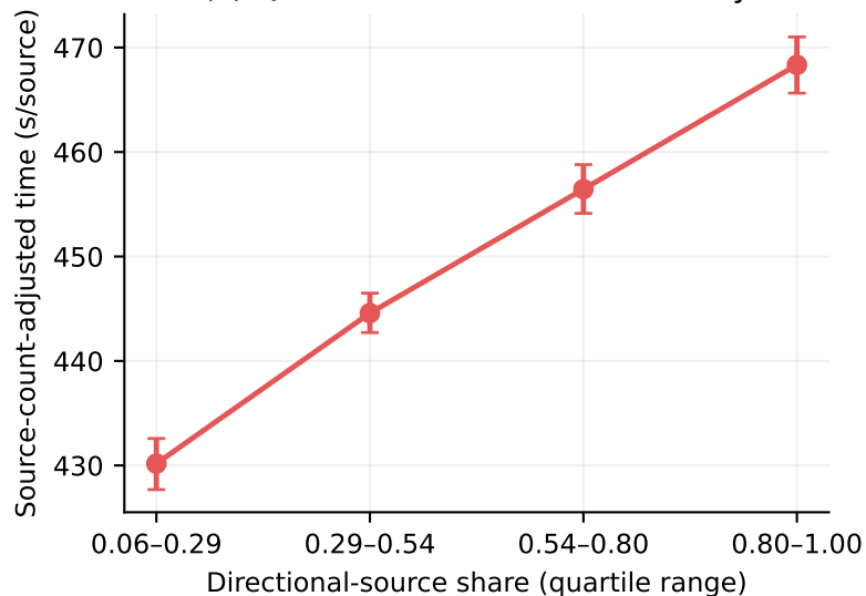
(c) Q4 directional-share sensitivity
