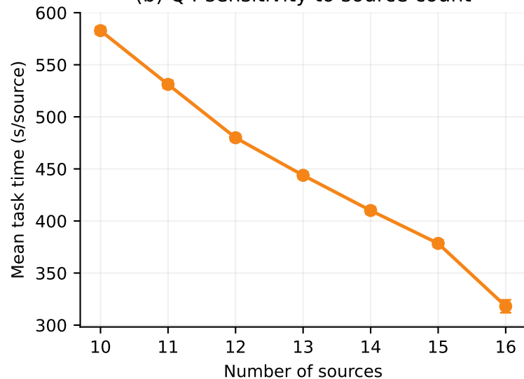
(b) Q4 sensitivity to source count
