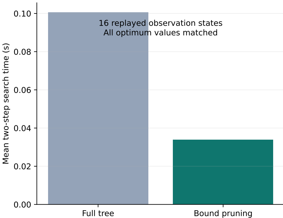
A. Same finite-tree optimum
