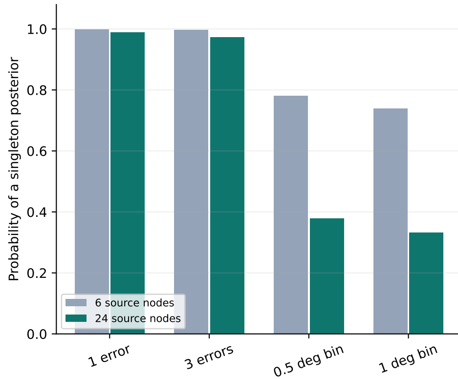
B. Discretization can invent certainty
