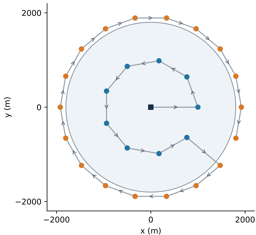
ring 28 3,744.5 s pure movement
