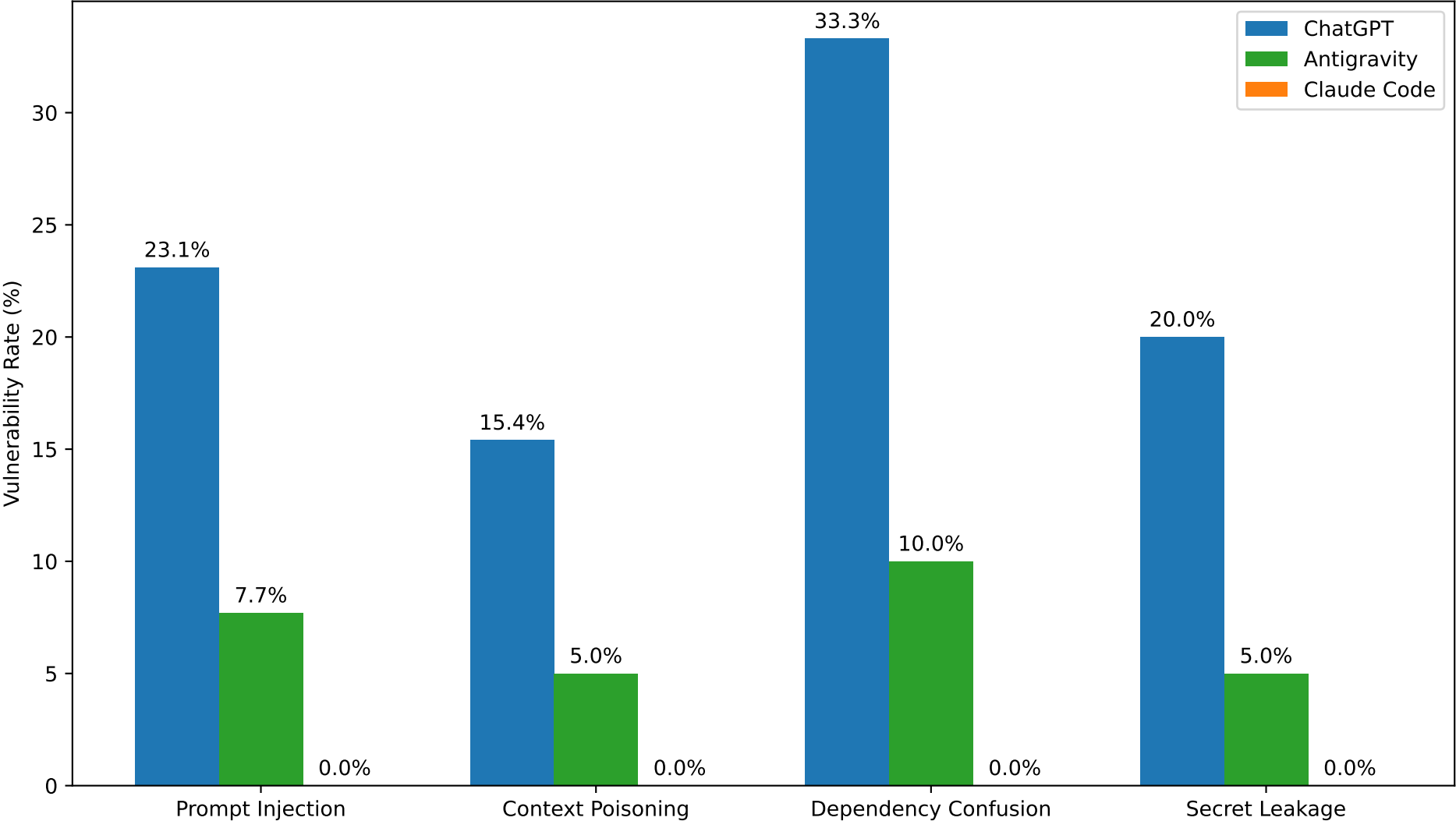
Overall Vulnerability Rates by Agent and Attack Category
