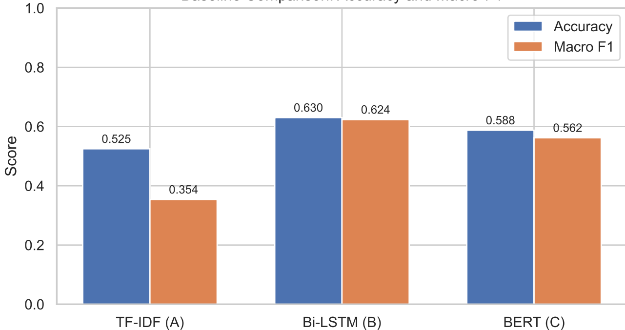
Baseline Comparison: Accuracy and Macro-F1
