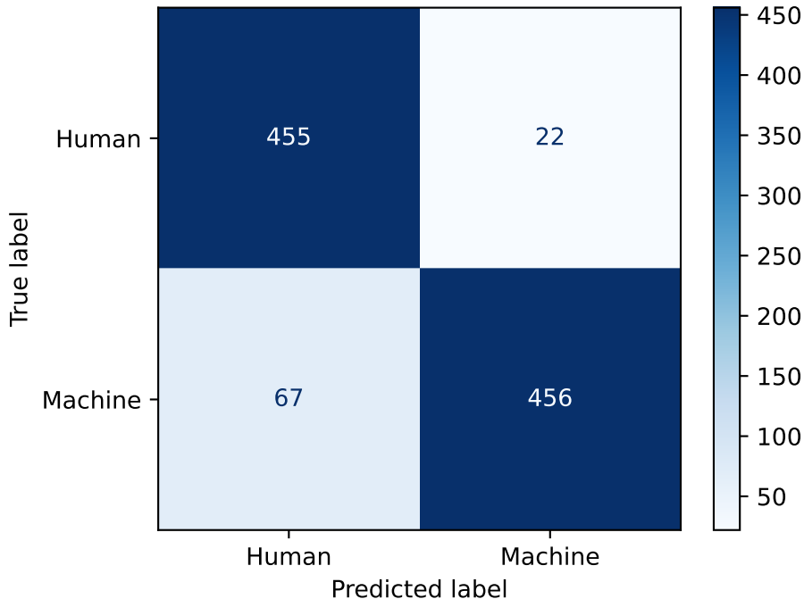
BERT-base Confusion Matrix (Test Set)
