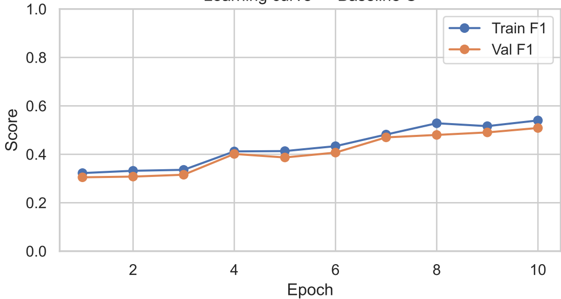
Learning curve — Baseline C
