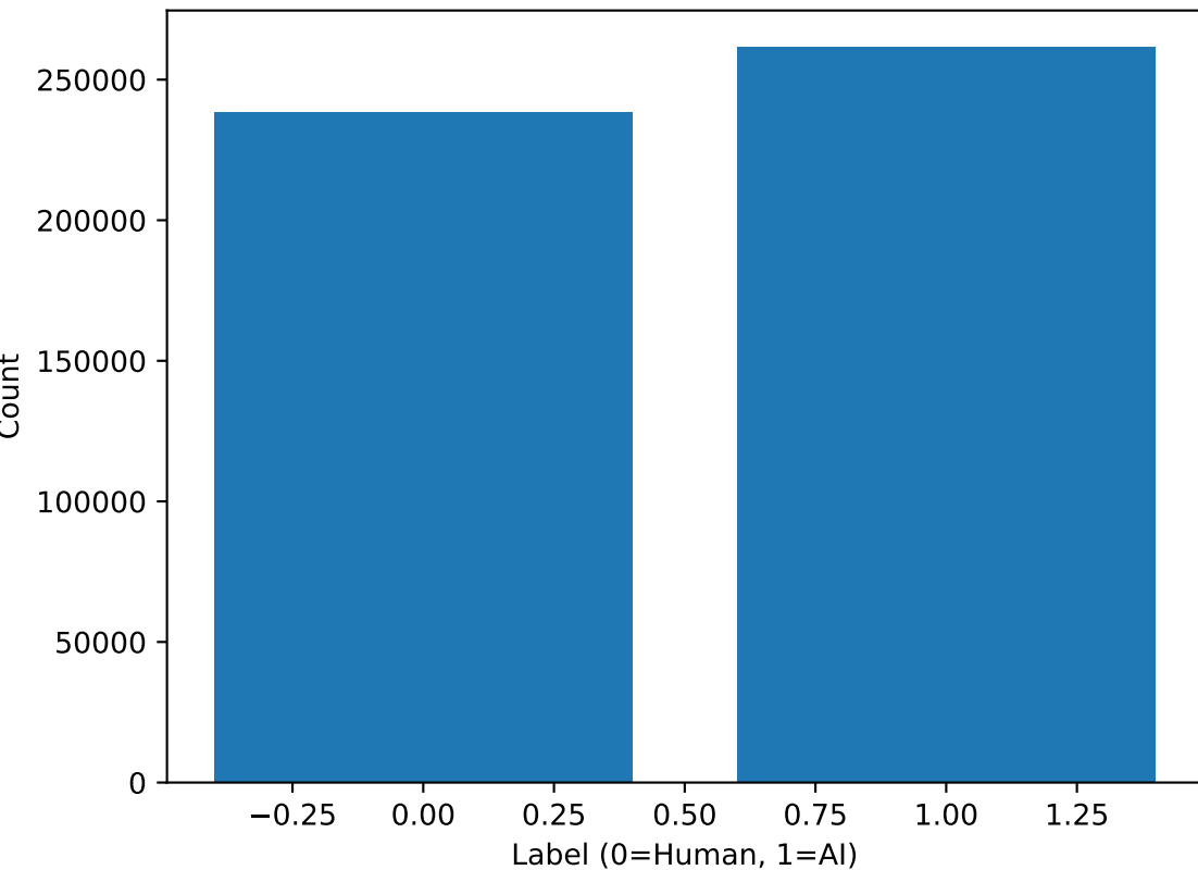
Label Distribution
