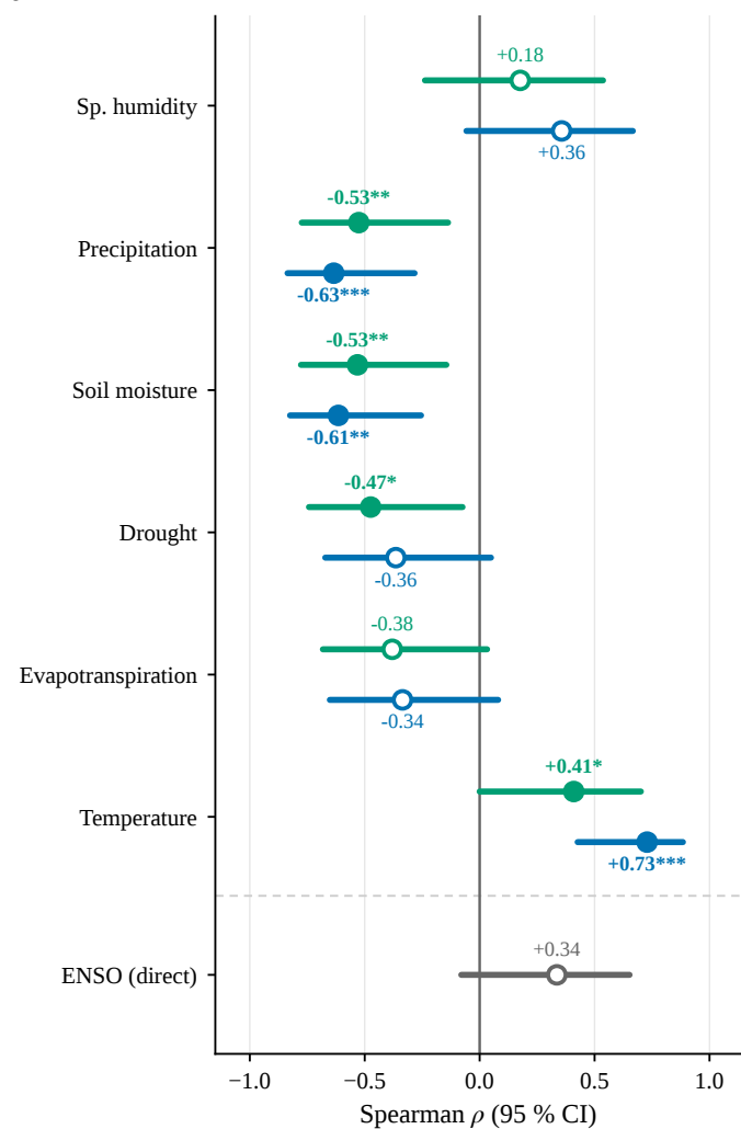
a ENSO → fire-season climate → area burned
