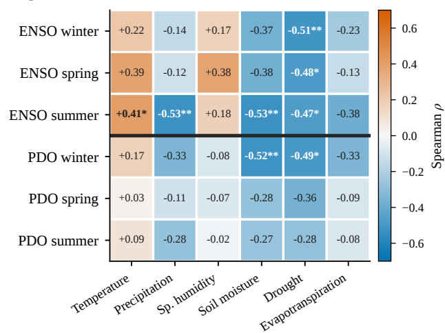
b ENSO and PDO vs fire-season climate
