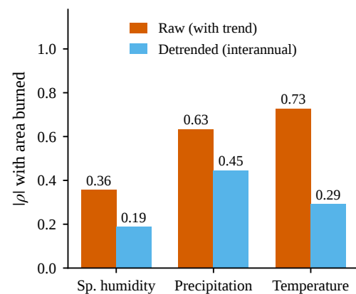
c Interannual vs trend control
