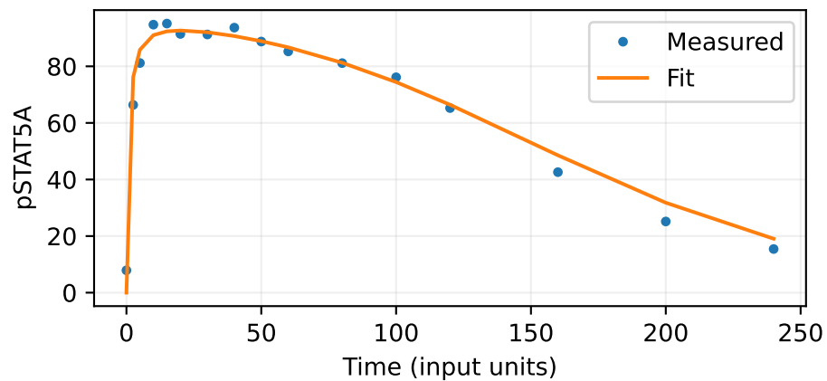
pSTAT5A RMSE = 4.409
