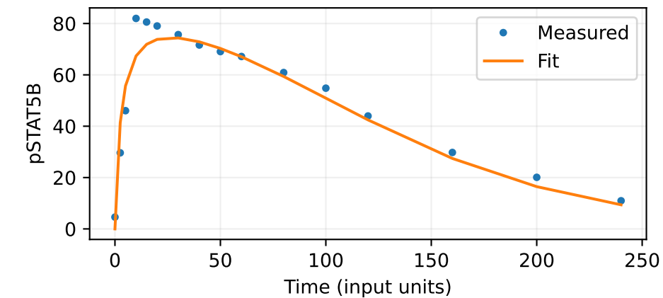
pSTAT5B RMSE = 6.193
