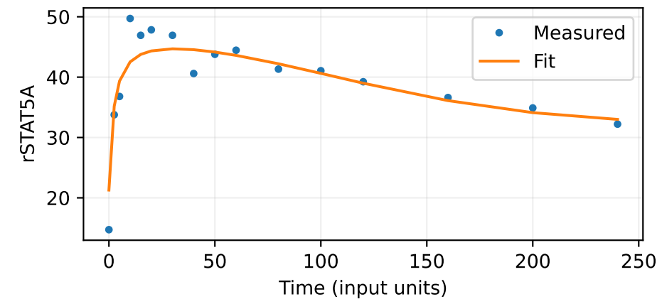
rSTAT5A RMSE = 3.058
