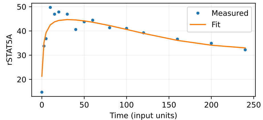
rSTAT5A RMSE = 3.058
