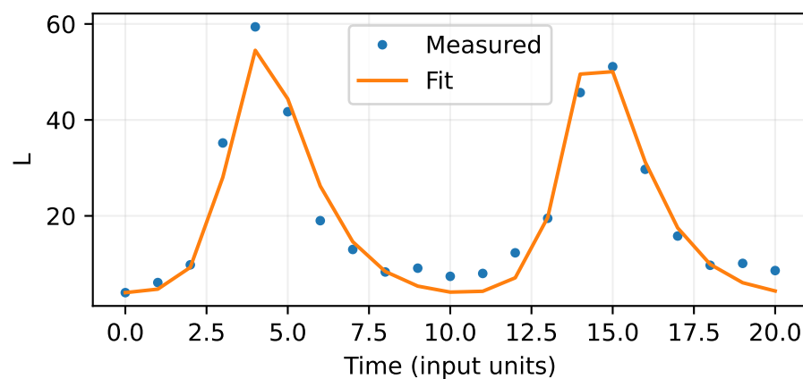
L RMSE = 3.525
