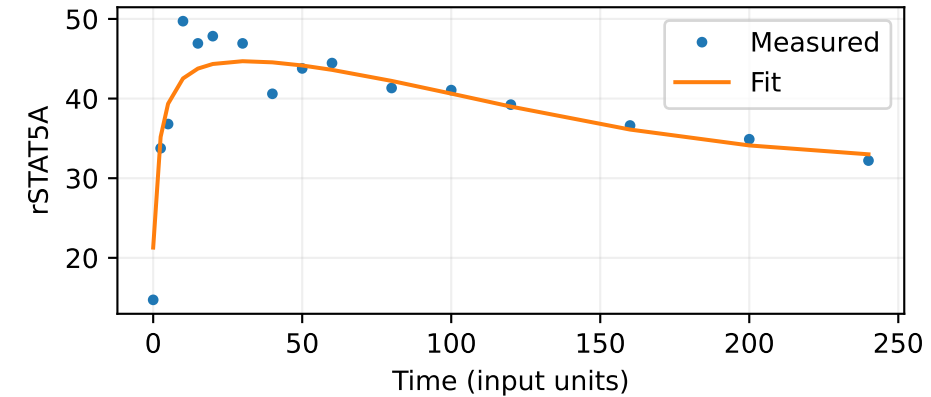
rSTAT5A RMSE = 3.058
