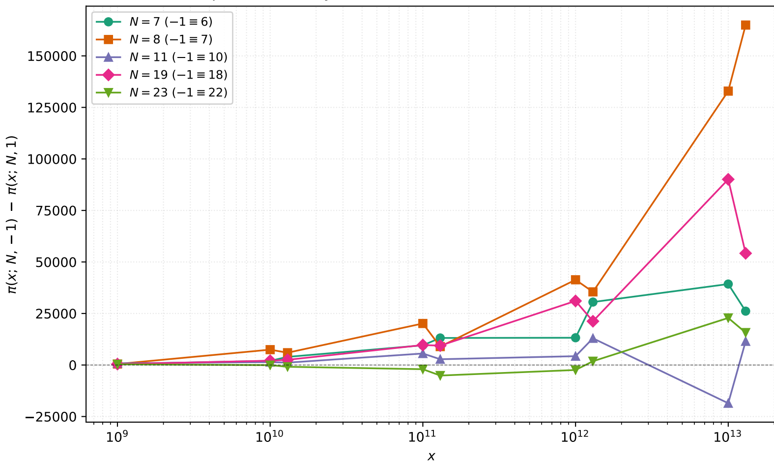
Replication of Koyama (2026): dominance of -1 \pmod{N} vs x
