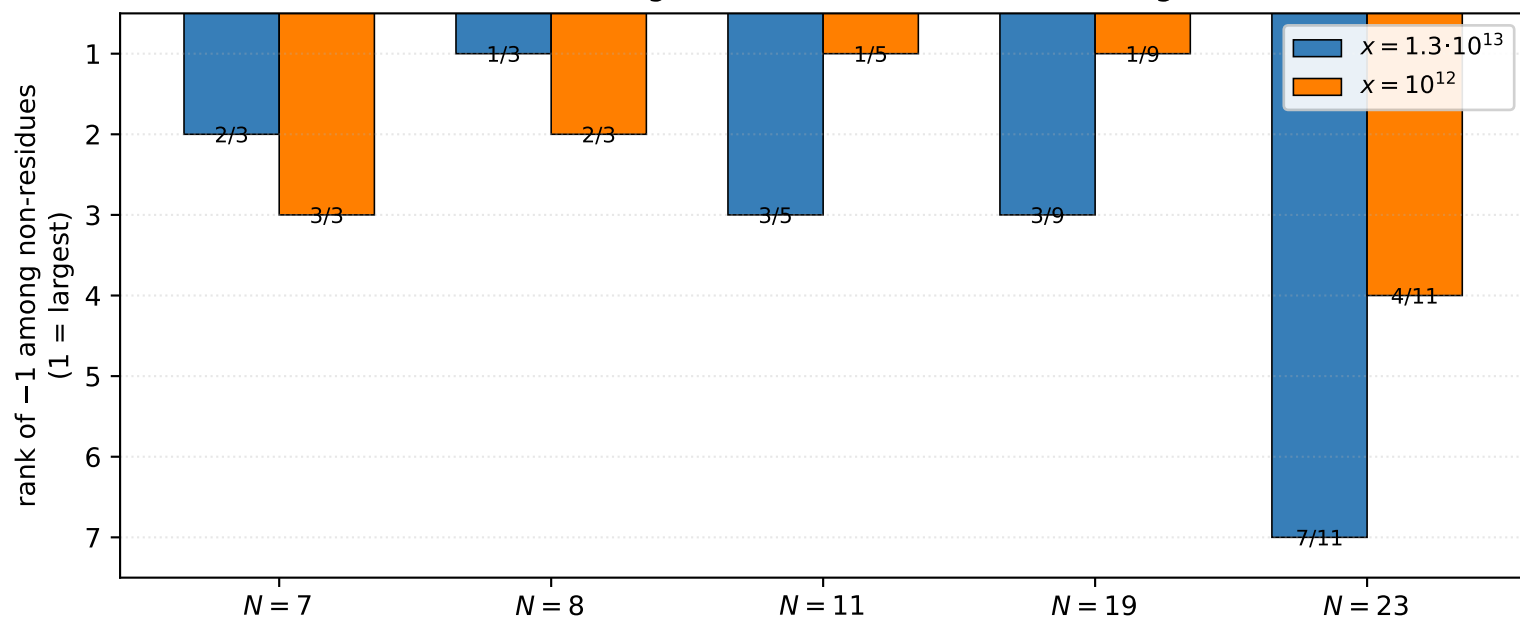
Rank of -1 \pmod{N} among non-residues (smaller = stronger dominance)
