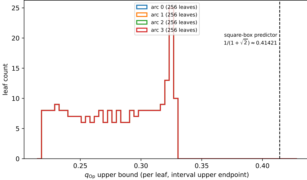
FIGURE 1. Per-arc distribution of qOp\_upper across the 1024 depth-8 leaves, arcs 0–3, with the square-box predictor 1/(1 + \sqrt{2}) \approx 0.41421 marked. Not yet rendered.
