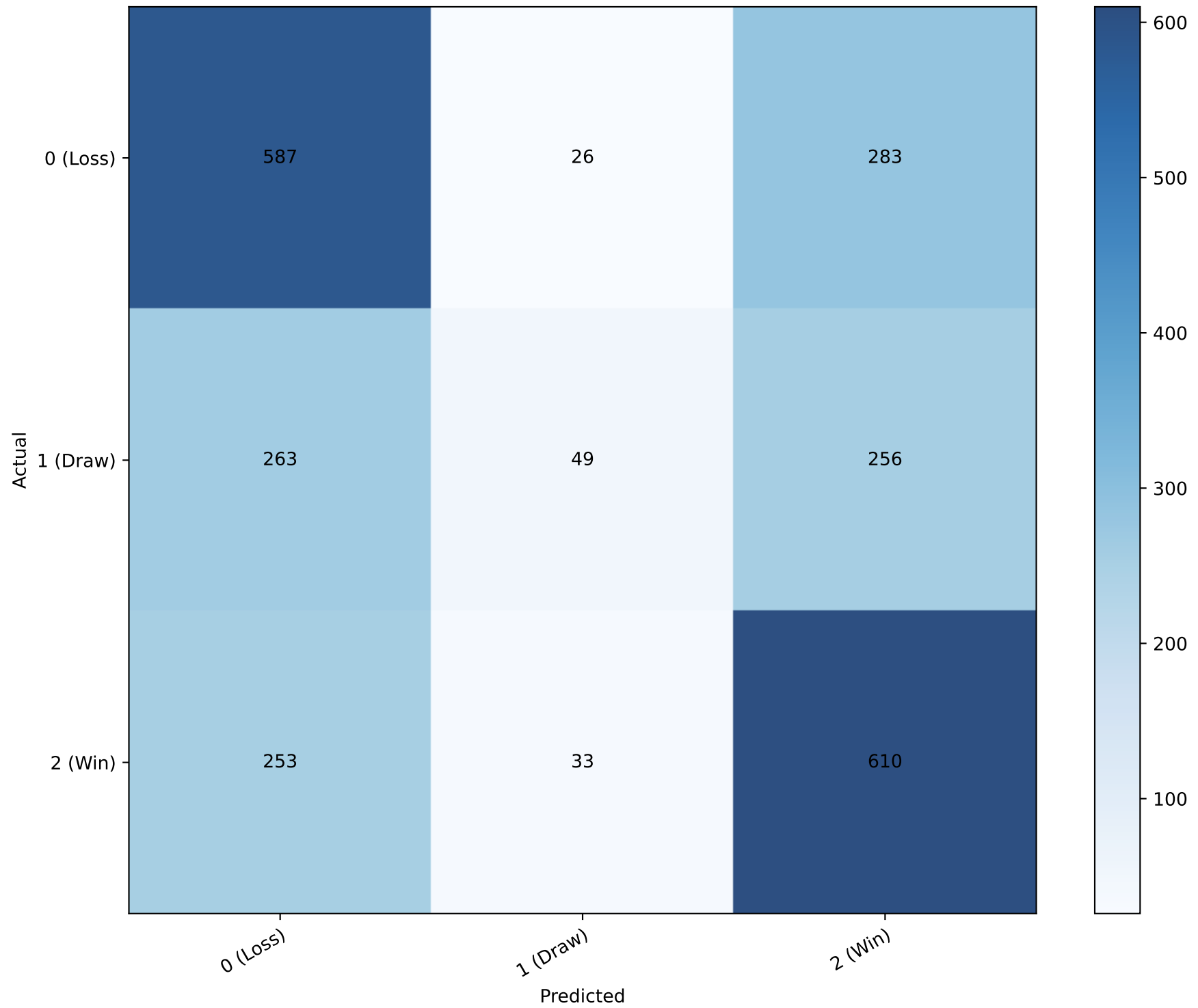
GradBoost — Confusion Matrix
