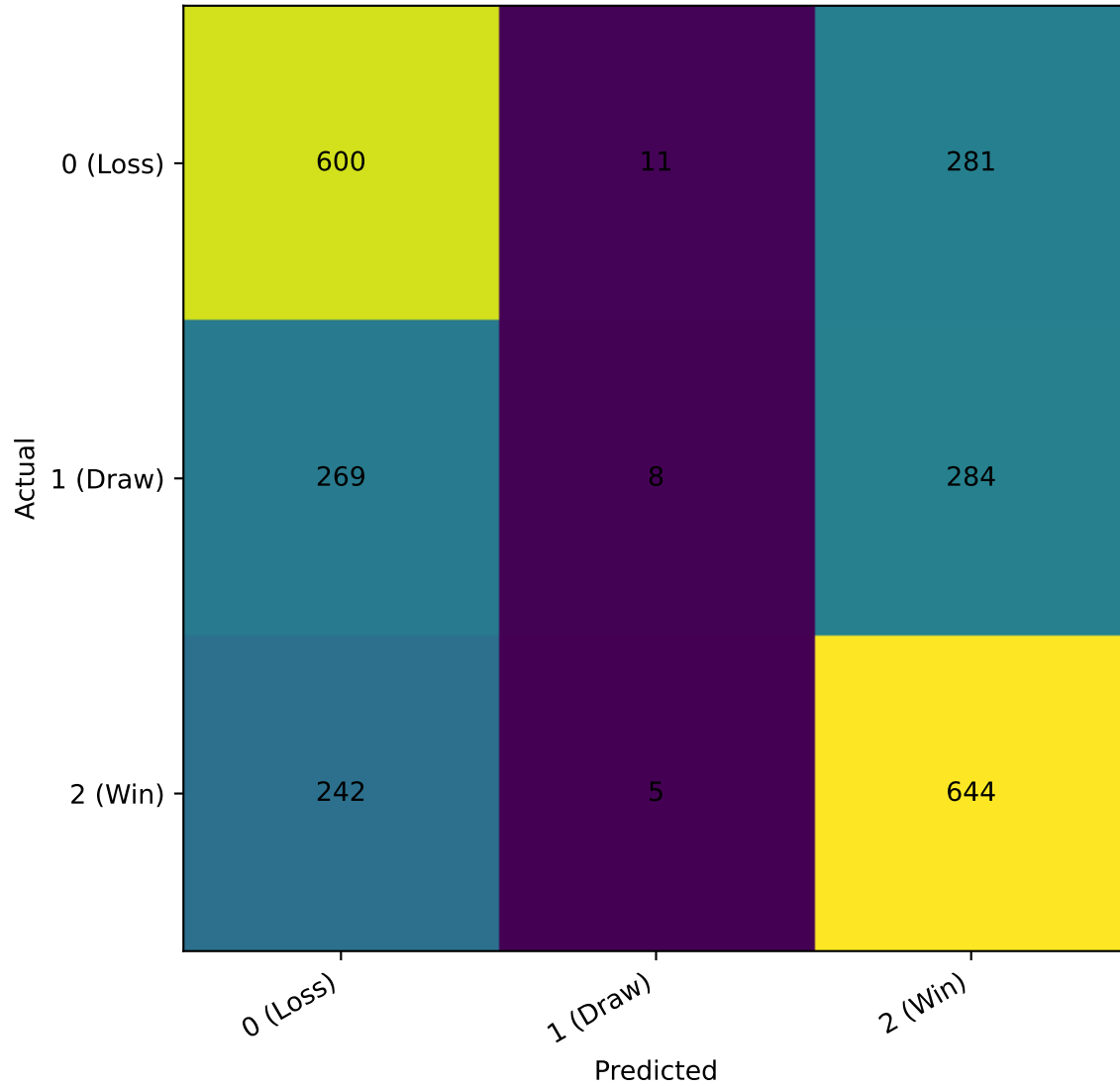
GradBoost — Confusion Matrix
