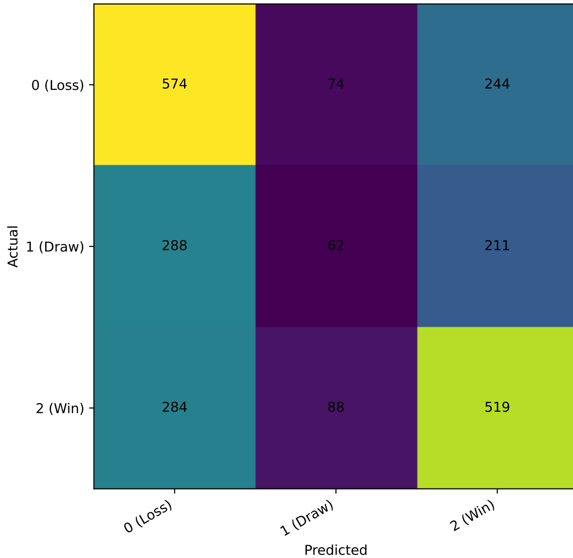
KNN — Confusion Matrix
