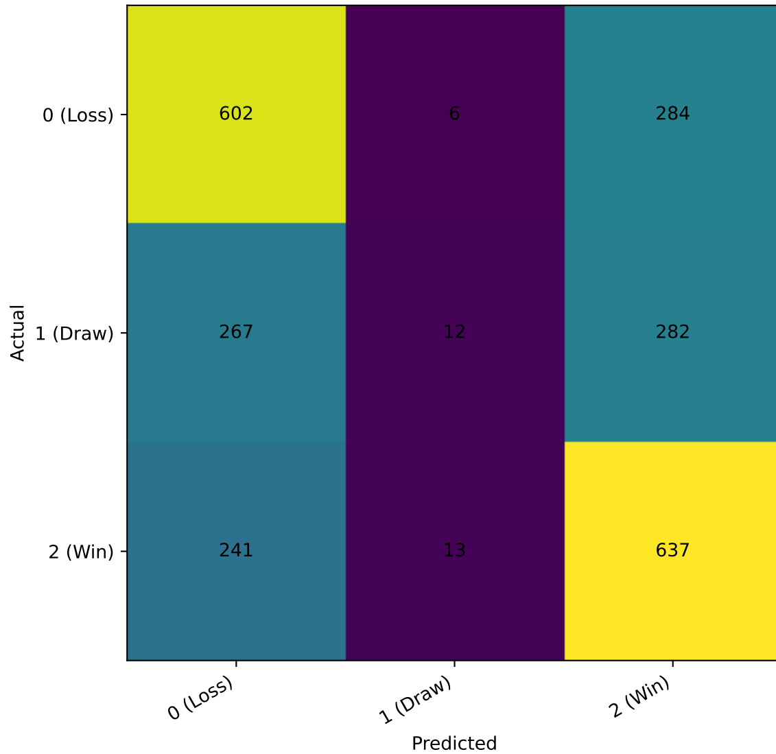
RandomForest — Confusion Matrix
