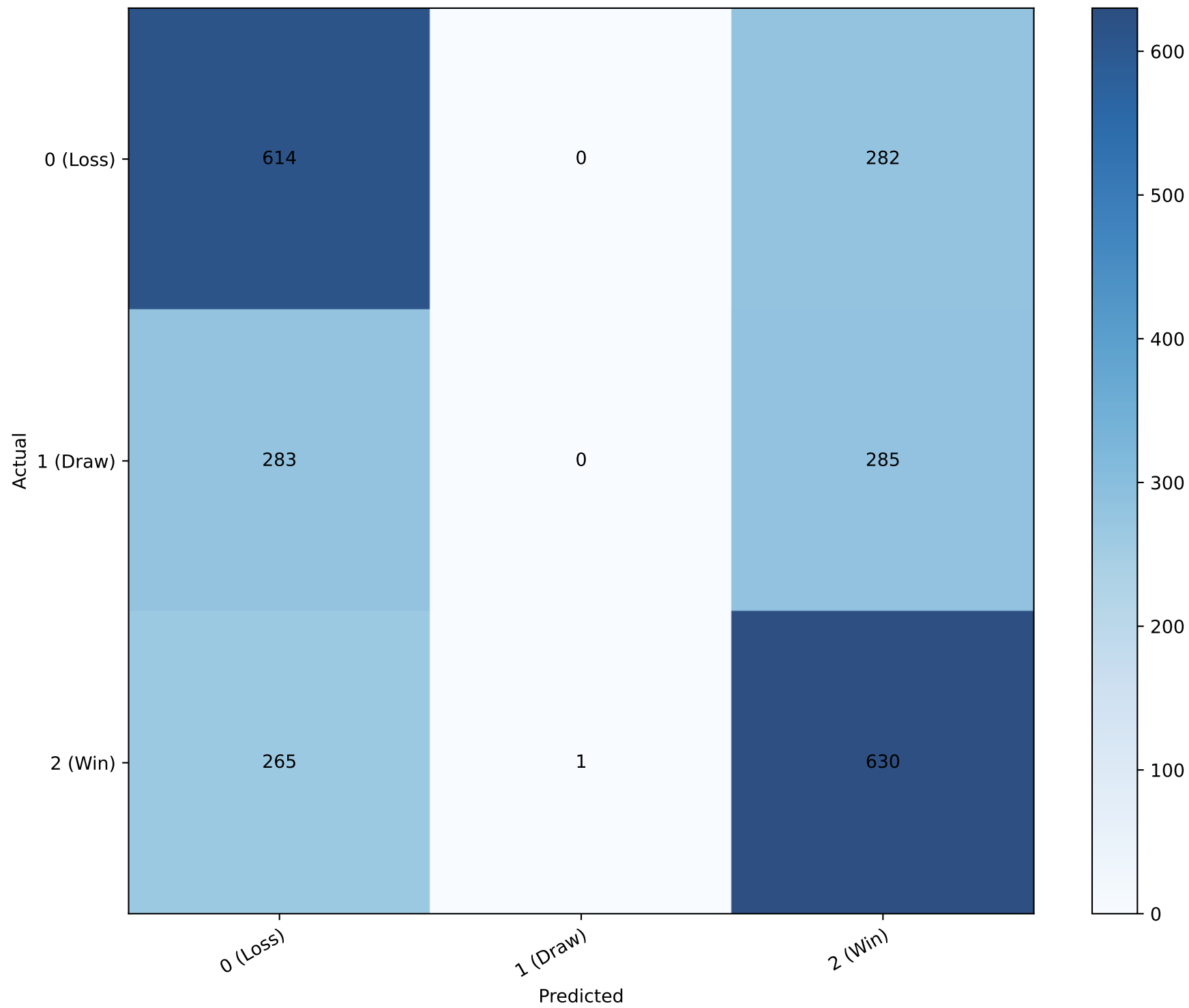
LogReg — Confusion Matrix
