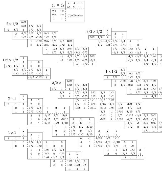
Figure 1: Clebsh-Gordan coefficients. A square root is understood on each coefficient, that is, -1/3 means -\sqrt{1/3} .
