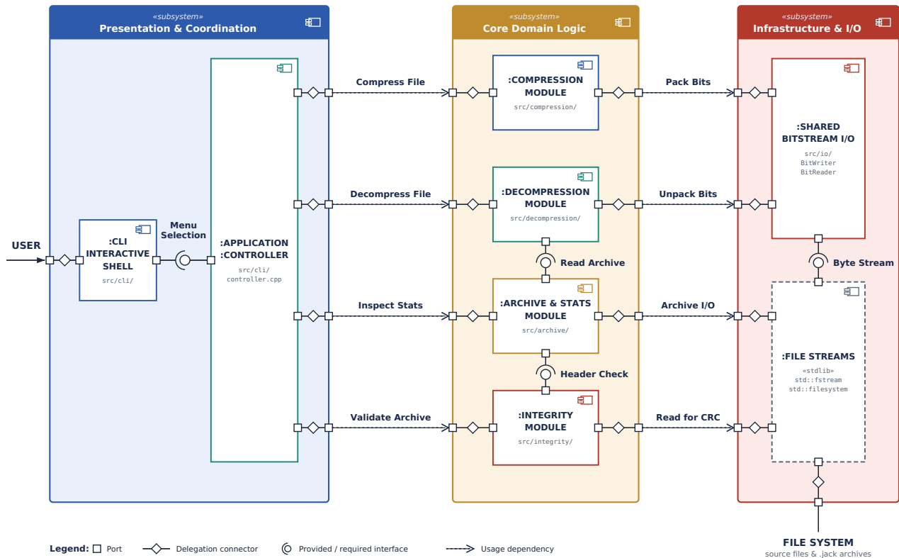
Fig. 2 — UML Component Diagram: subsystems, ports, interfaces and usage dependencies
