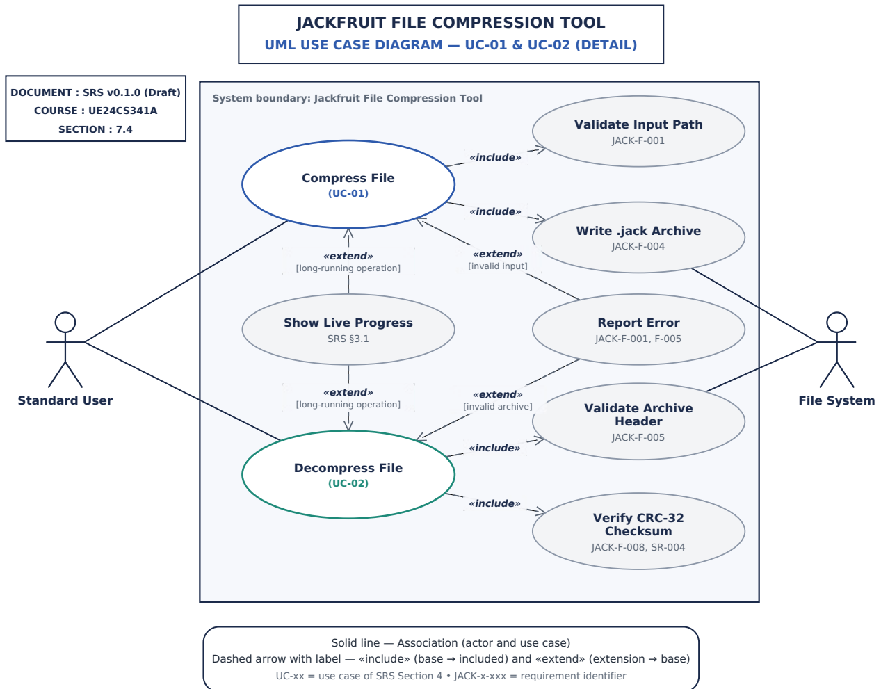
Fig. 5 — Use-Case Diagram 4: Compression and decompression in detail
