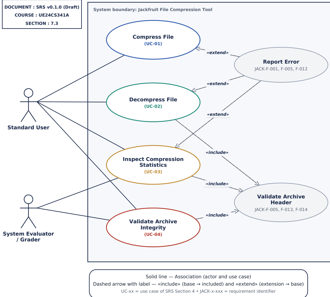
Fig. 4 — Use-Case Diagram 3: System overview with actors, «include» and «extend»
