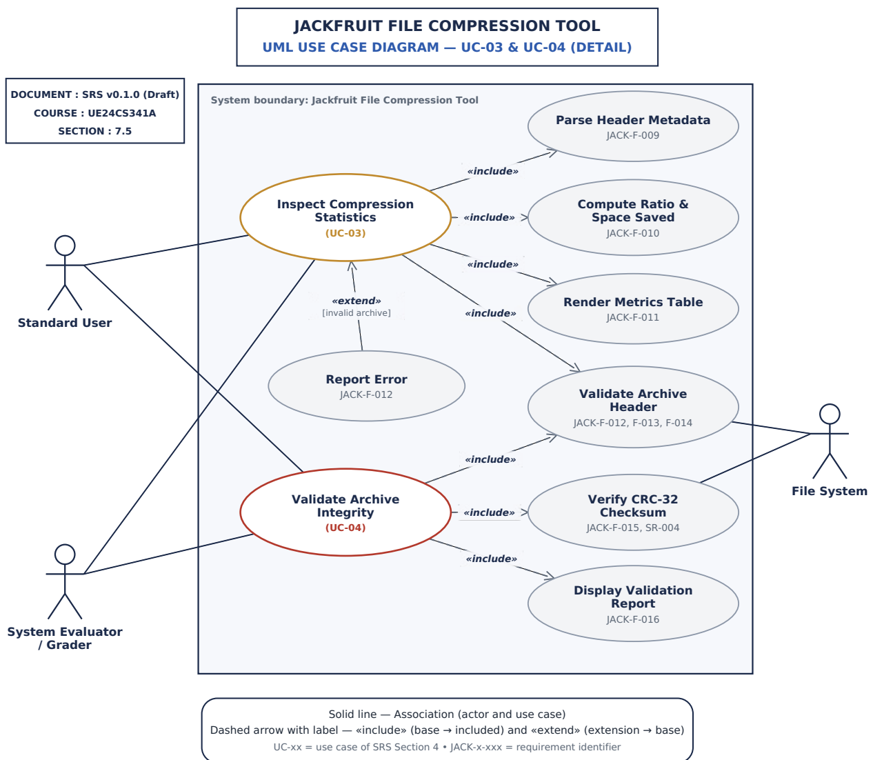
Fig. 6 — Use-Case Diagram 5: Statistics and validation in detail
