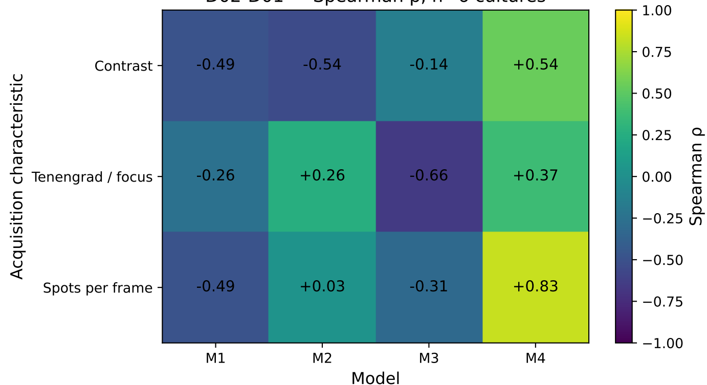
Association between acquisition changes and prediction changes D02-D01 — Spearman \rho , n=6 cultures
