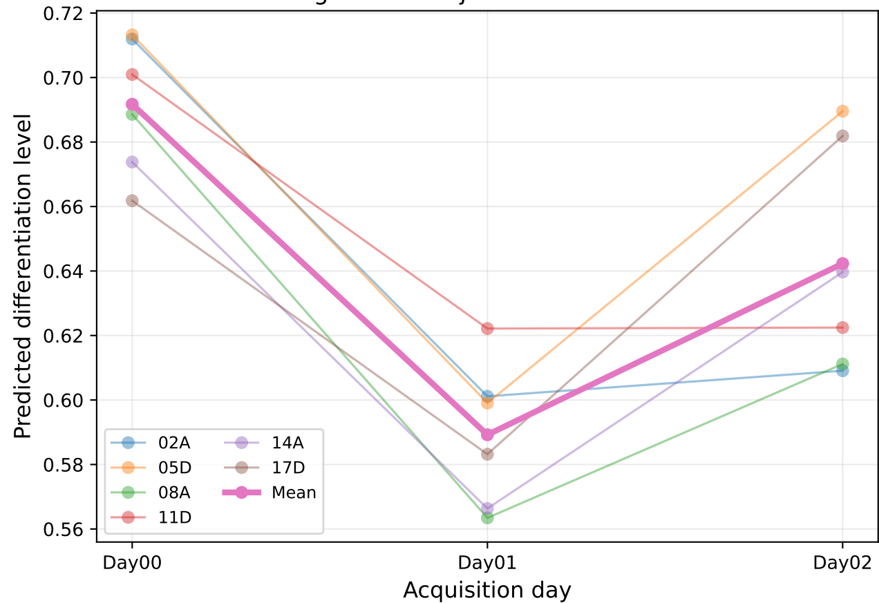
M3 — longitudinal trajectories across 6 cultures
