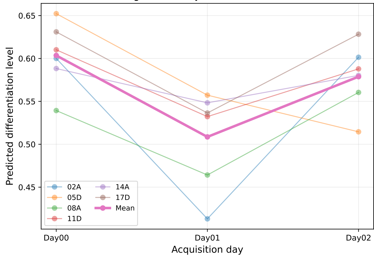
M4 — longitudinal trajectories across 6 cultures
