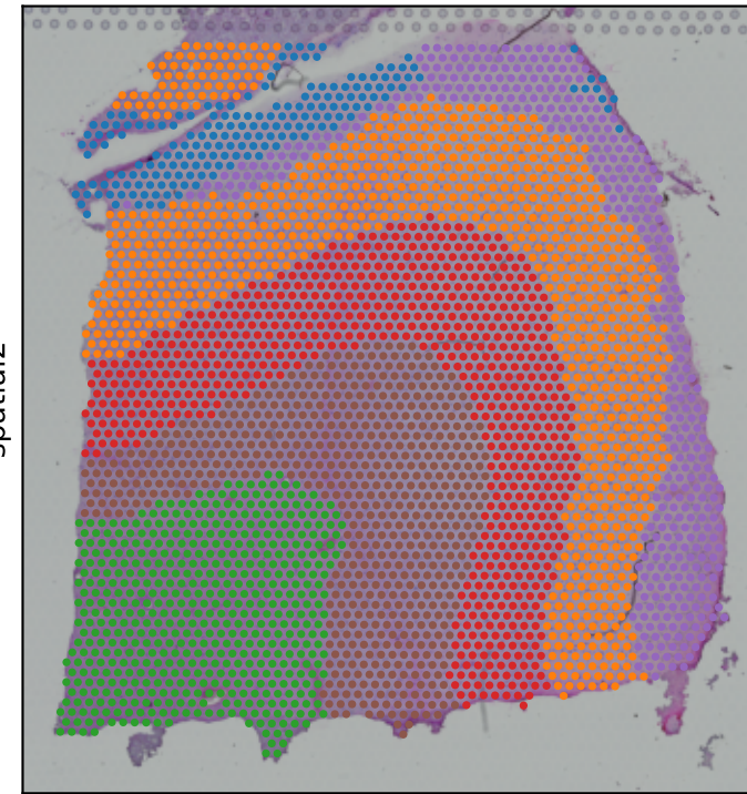
ARI=0.6371
