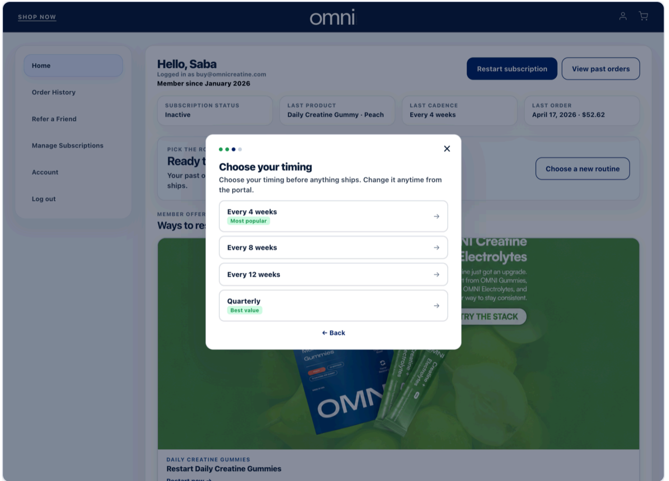
Step 3 — cadence.
