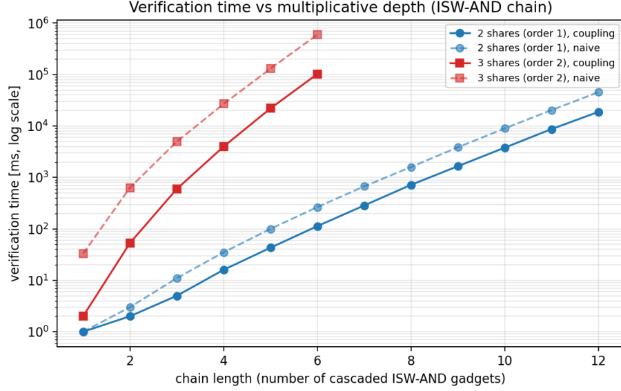
Figure 7.1 Verification time versus circuit depth
