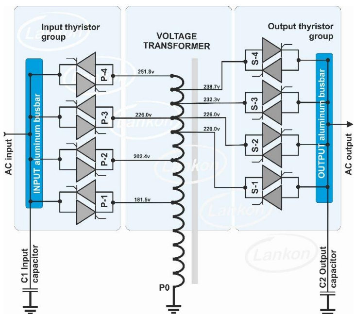
Figure 8 — Static Voltage Regulator Operating Principle Diagram
