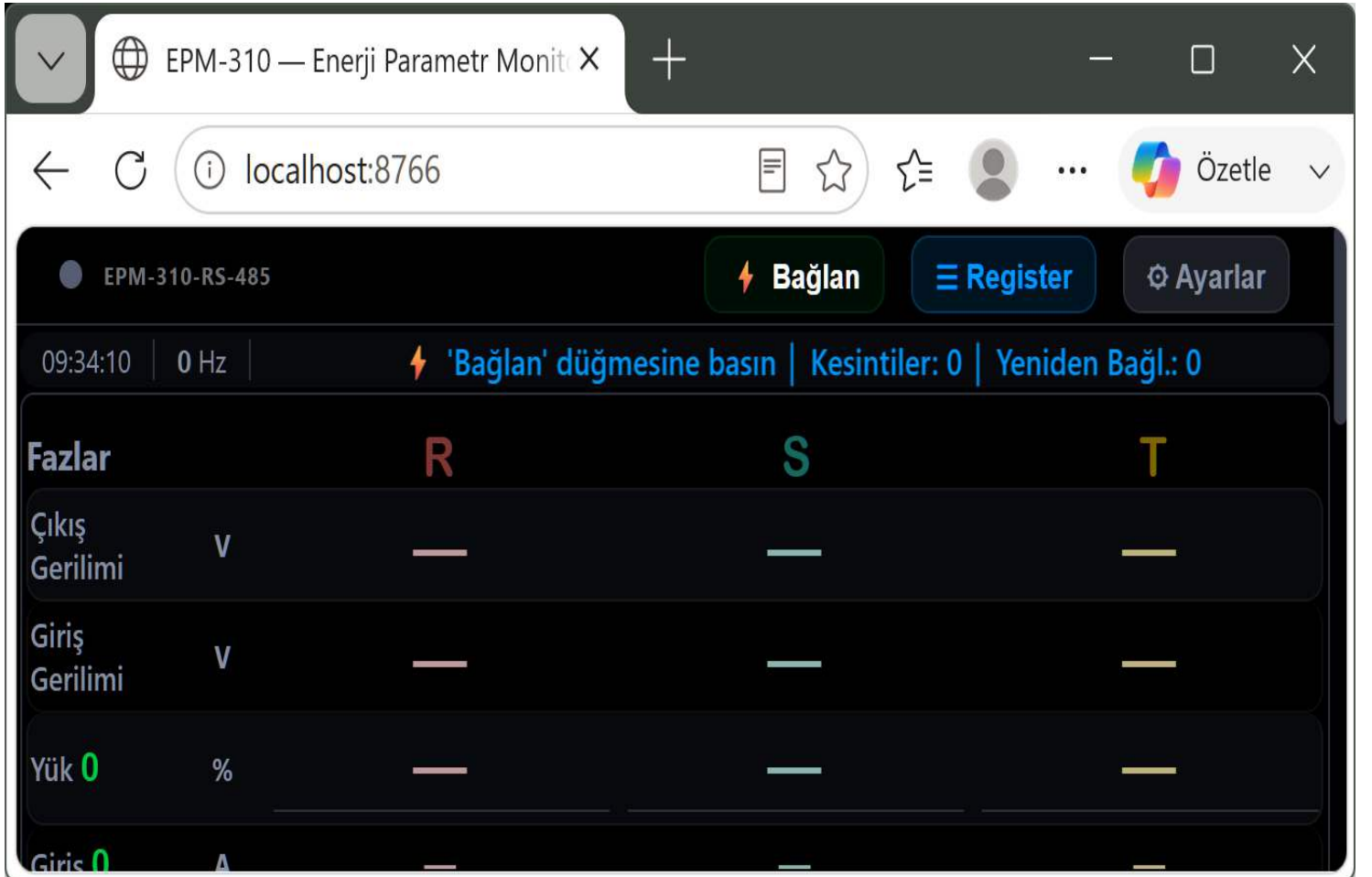
Şek. 2 — Ana panel EPM-310-RS-485 (http://localhost:8766/)
