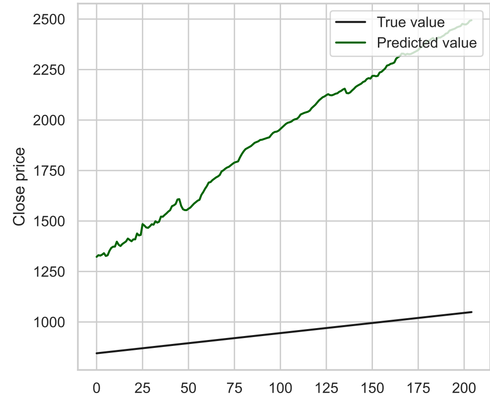
(a) LSTM - Test Data
