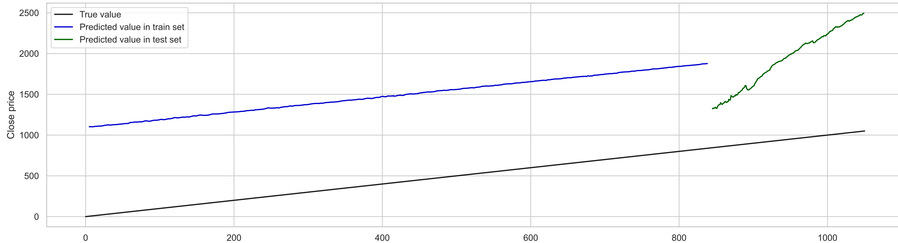
LSTM Model - Full Data Predictions
