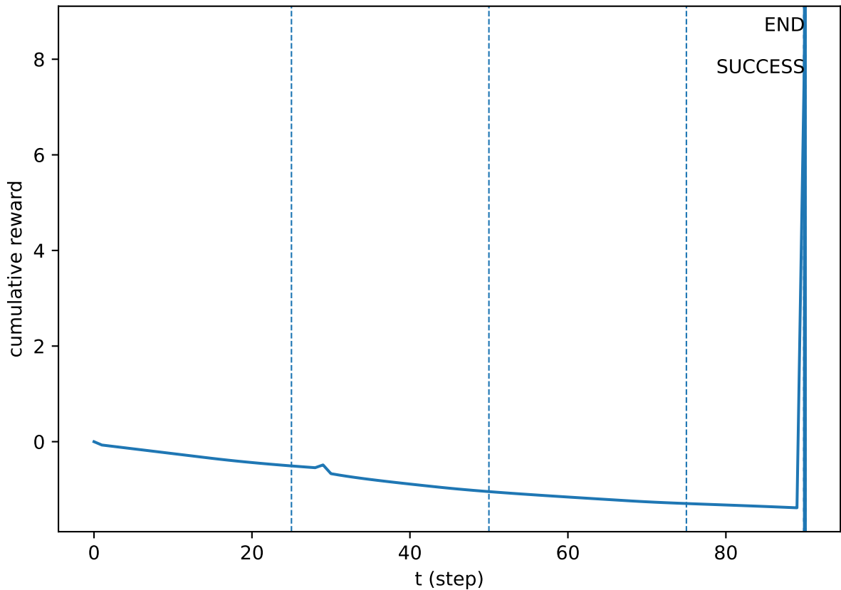
Cumulative Reward
