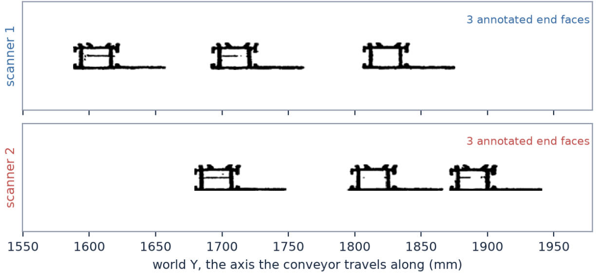
Figure 2.3: The same bundle seen from the two ends. YZ projection on which the two detectors operate for the same scene. The two views are drawn on the same Y-axis of the world reference frame, making the face positions directly comparable. The faces are identical up to the saw marks but the two views do not coincide along Y because the conveyor belt moves between the two acquisitions. The scene belongs to the L-profile family.
