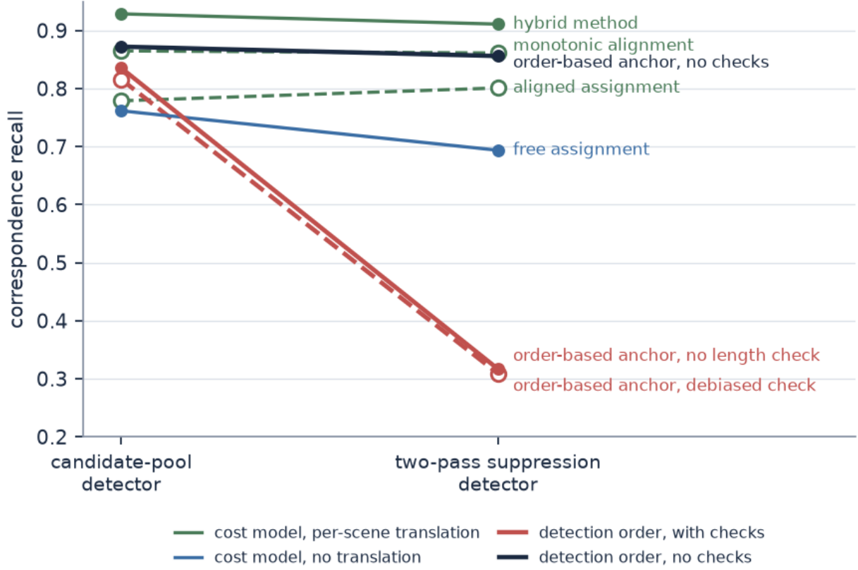
Figure 5.1: Effect of a change of detector. Correspondence recall for each method across the two detectors using identical ground truth and scene sets. Colours distinguish four methodological groups: methods using the shared cost model with a per-scene translation estimate, free assignment (which employs the cost model without a translation estimate), the two order-based anchors retaining acceptance checks from the original system and the check-free order-based anchor. Dashed lines with open markers serve solely to resolve visually overlapping trajectories. Only the two anchors with acceptance checks lose most of their recall, whereas the order-based anchor without checks remains as stable as the cost-model methods.
