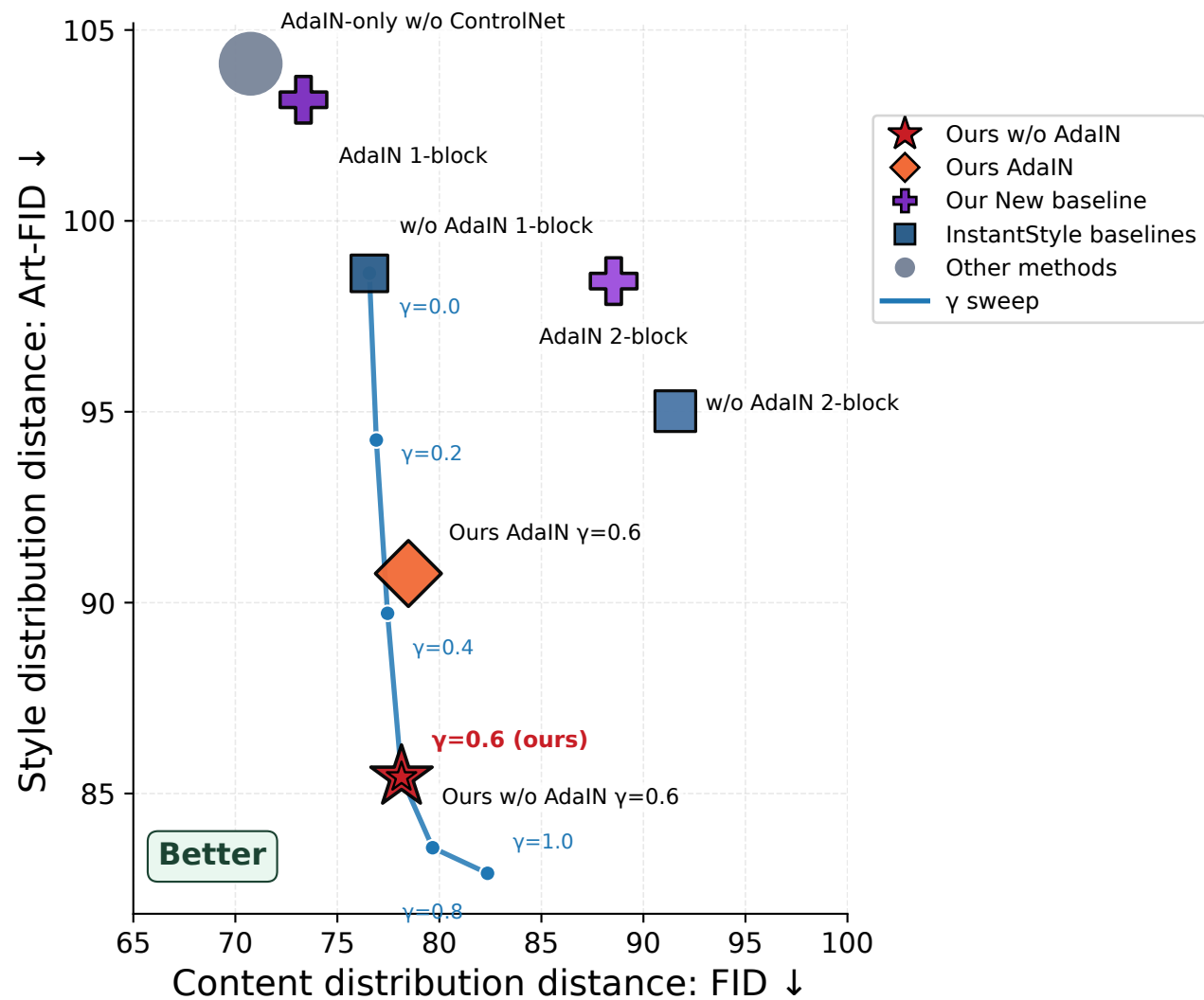
Content-Style Trade-off on 5k Evaluation Set
