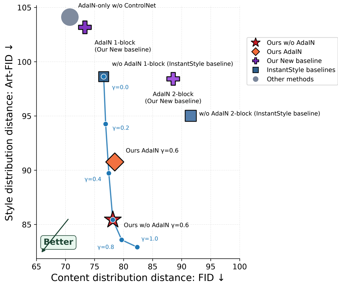
Content-Style Trade-off on 5k Evaluation Set
