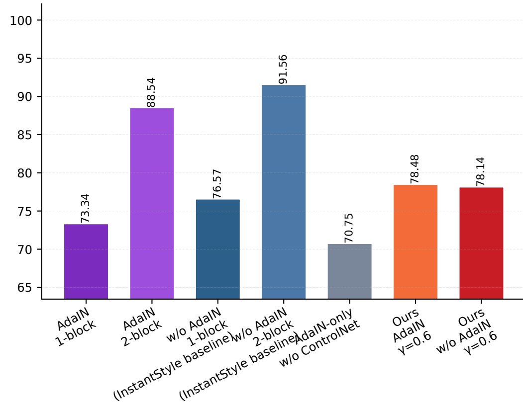
(a) FID ↓
