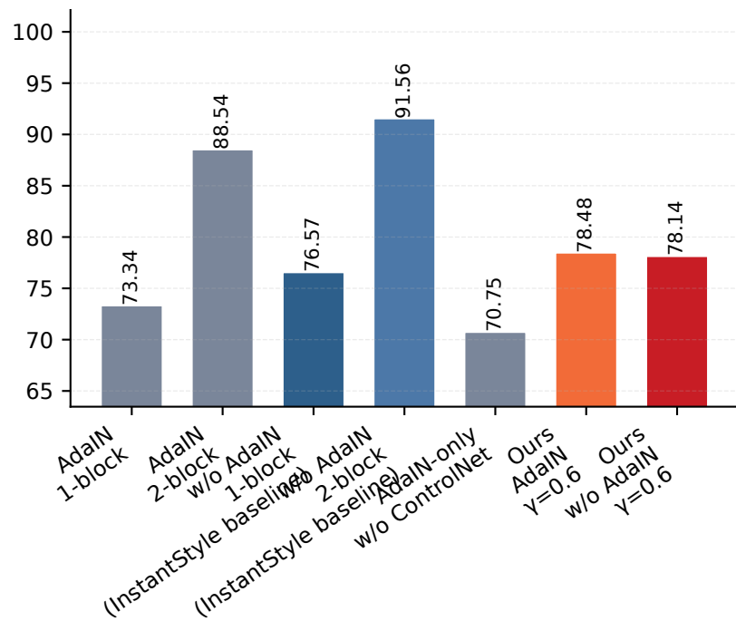
(a) FID ↓
