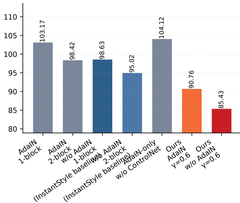
(b) Art-FID ↓
