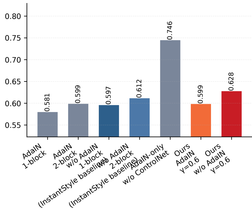
(c) LPIPS ↓
