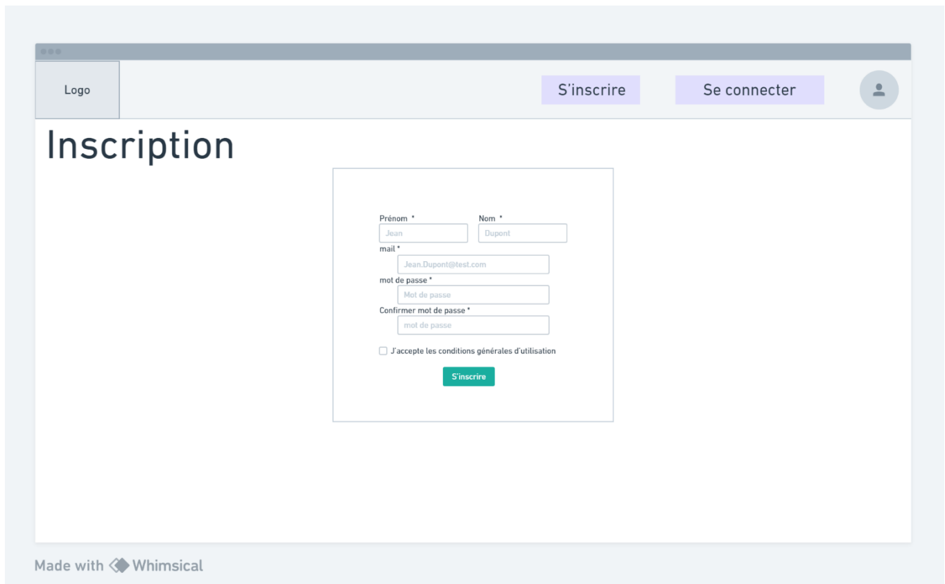
Figure 2.12 – Wireframe – Inscription
