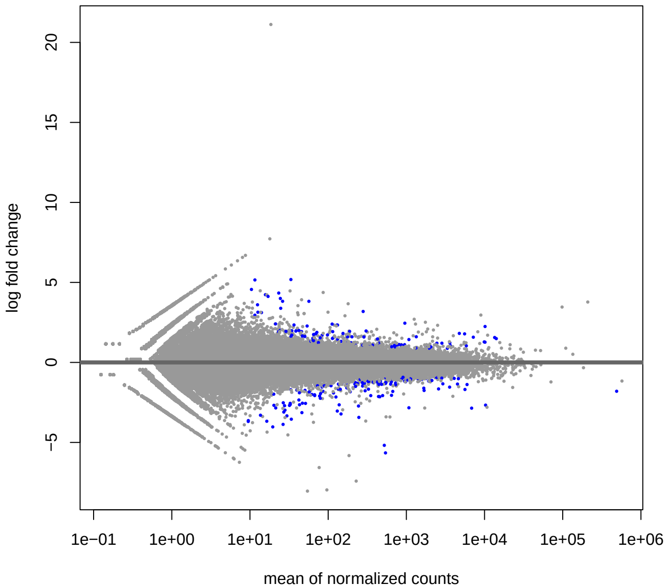
MA-plot for Condition: Normal vs TNB
