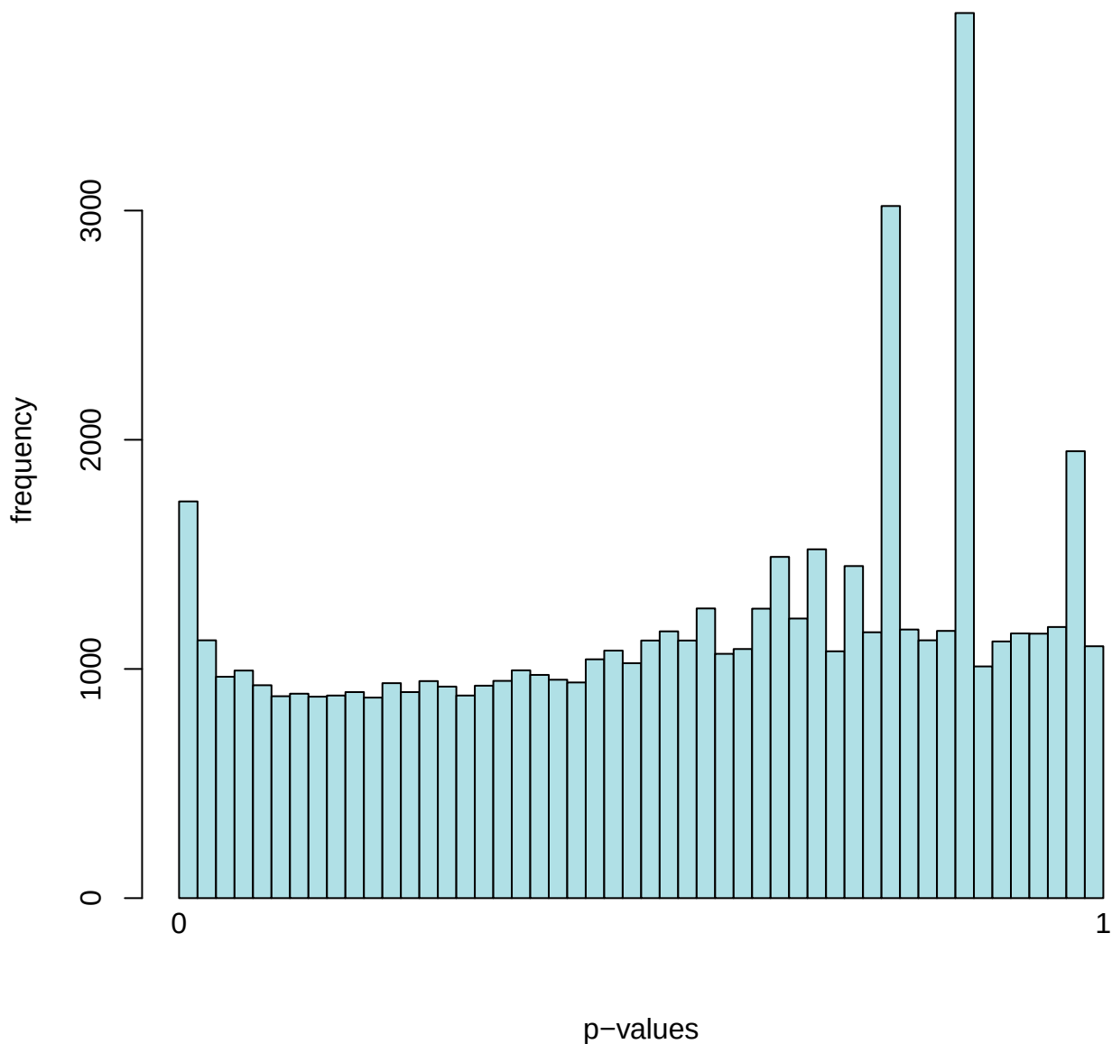
Histogram of p-values for Condition: Normal vs TNB
