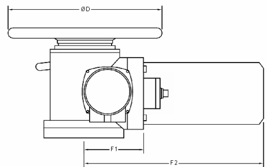
FIG- LEFT SIDE VIEW
