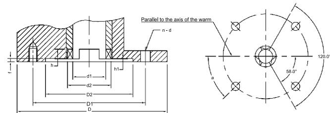
FIG- ACTUATOR MOUNTING
