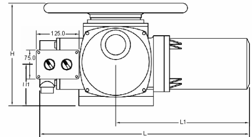
FIG- FRONT VIEW
