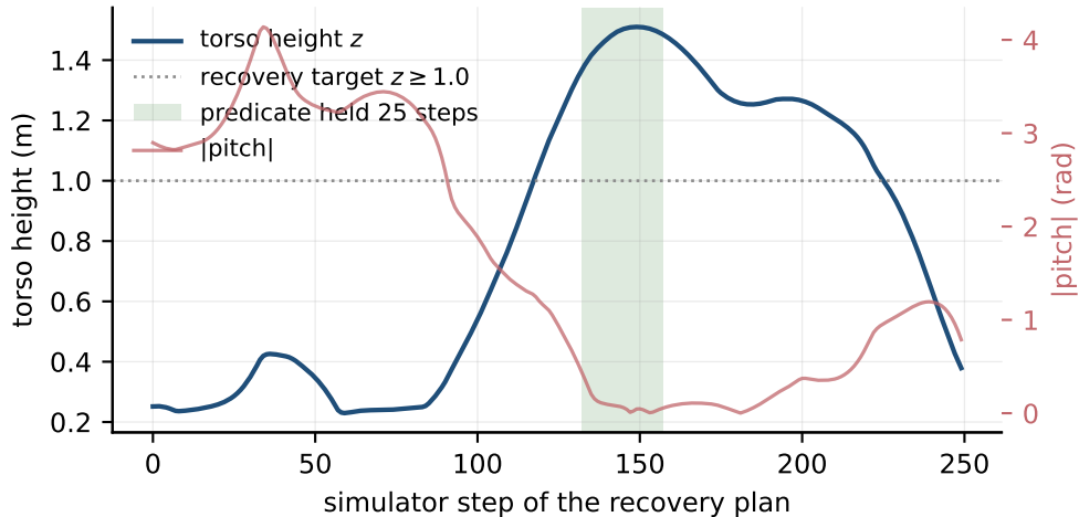
Walker2d standing up from z = 0.25 , pitch -2.92 rad
