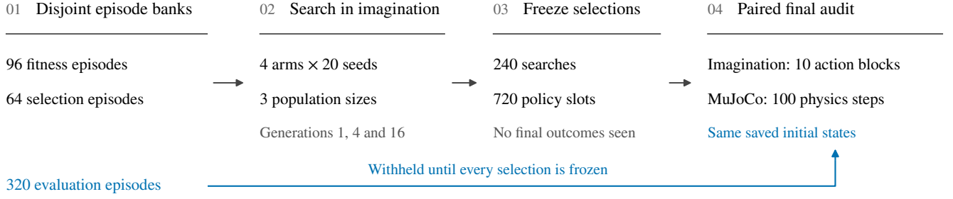
Figure 2: Locked study design. Episodes are disjoint across roles, with one start state per episode. All selections were frozen before final evaluation. In imagination, controllers act on predicted latents; in MuJoCo, on newly rendered images. Paired start states therefore do not imply identical action sequences.
