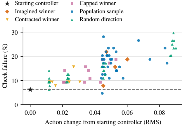
Figure 6: Exploratory audit of 89 fixed controllers on 64 reused check episodes. Failure rises with how far a candidate changes the starting controller’s actions on the same inputs. The dashed line is the starting controller.
