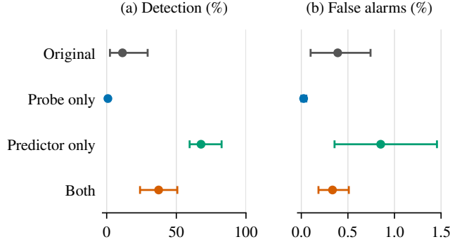
Figure 7: Exploratory repair audit: 24 reused source episodes, 89 fixed candidates. Points average the three fitting seeds for repaired arms; whiskers are source-episode bootstrap 95% intervals. Detection is at the first unsafe block endpoint, not an advance warning. False alarms use still-healthy endpoints. Predictor-only repair passes the frozen gate.
