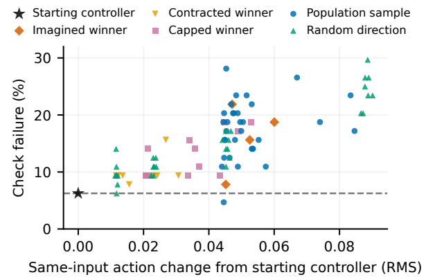
Figure 6: Exploratory audit of 89 fixed controllers on 64 reused check episodes. Failure rises with how far a candidate changes the starting controller’s actions on the same inputs. The dashed line is the starting controller.
