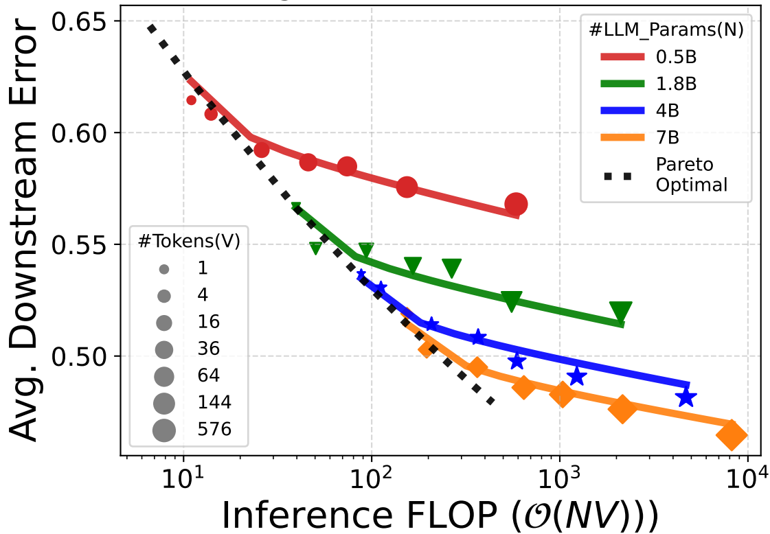
Scaling #Params vs #Visual Token
