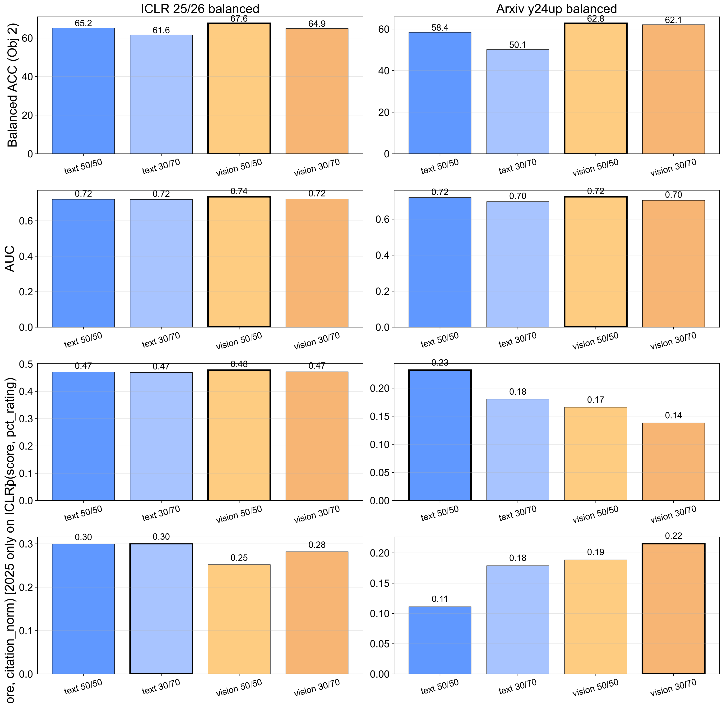
Modality × train-ratio comparison: 7B 2nd-ckpt models on ICLR 25/26 + arxiv y24up balanced
