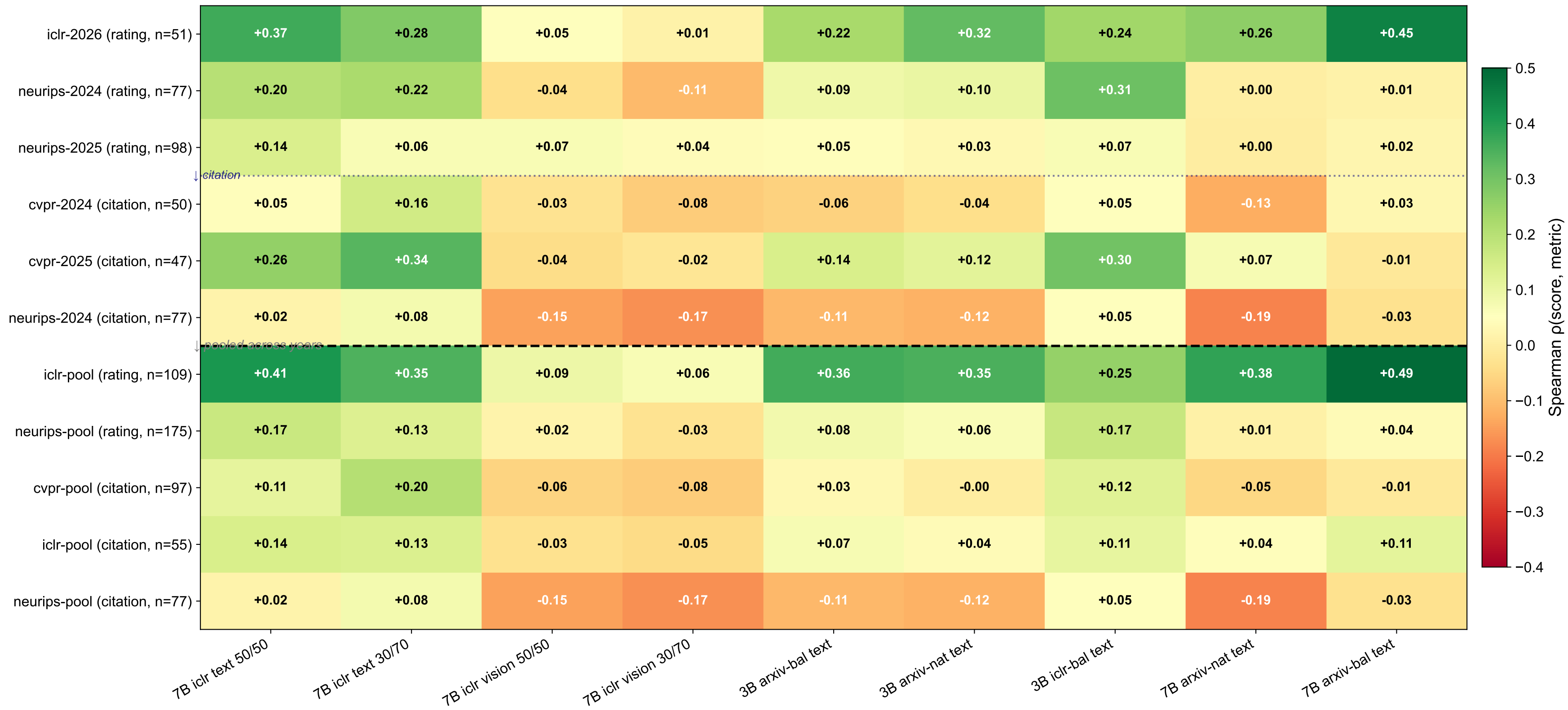
Per-(venue, year) Spearman \rho(\text{score}, \text{quality\_signal}) — arxiv balanced test Rows: cells with \geq 40 samples for the signal. Top half: per-year. Bottom: pooled.
