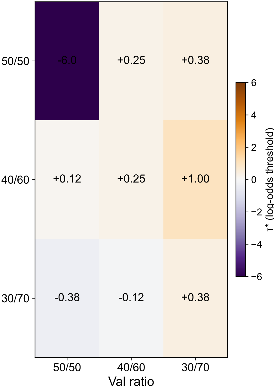
ICLR \tau^* threshold from val
