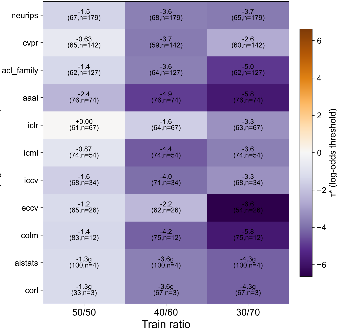
Arxiv per-venue \tau^* from val (val acc / n)
