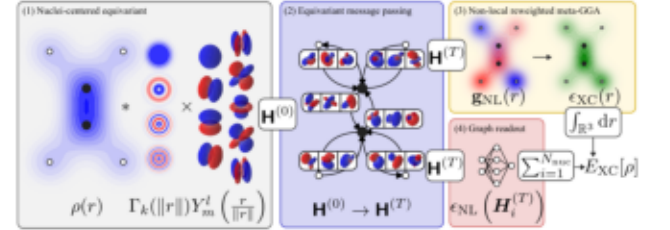
Figure 1: Illustration of Equivariant Graph Exchange Correlation (EG-XC)’s four components: (1) We obtain a finite atomic-range point cloud representation \mathbf{H}^{(0)} by convolving the electron density \rho with radial filters \Gamma_k : \mathbb{R}_+ \rightarrow \mathbb{R} and spherical harmonics Y_m^l : \mathbb{R}^3 \rightarrow \mathbb{R} at the nuclear position. (2) The embeddings \mathbf{H}^{(0)} are updated using equivariant message passing to obtain molecular-range effects in \mathbf{H}^{(T)} . (3) We define a non-local feature density g_{\text{NL}} : \mathbb{R}^3 \rightarrow \mathbb{R}^d from which we derive the exchange correlation density \epsilon_{\text{XC}} : \mathbb{R}^3 \rightarrow \mathbb{R} . (4) We add a graph readout of \mathbf{H}^{(T)} to learn additional corrections. To obtain E_{\text{XC}}[\rho] , we integrate \epsilon_{\text{XC}} and add it to the global graph readout.
