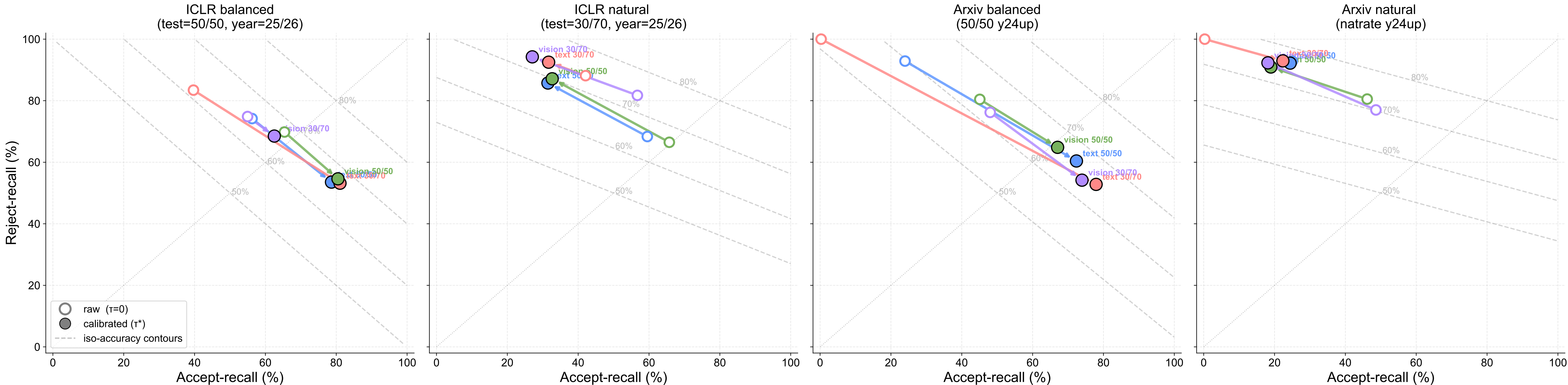
Calibration trades reject-recall for accept-recall — open \square filled (TEST split, 7B)
